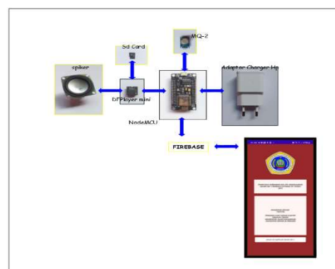
Gambar 6. Block Diagram
