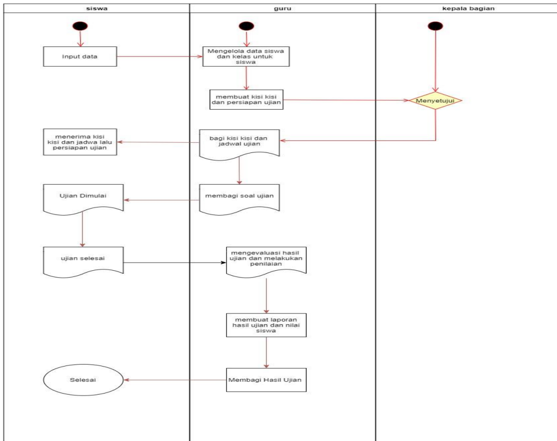
Gambar 3. Activity Diagram
