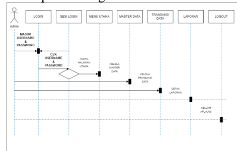
Gambar 2. Sequence Diagram Admin
