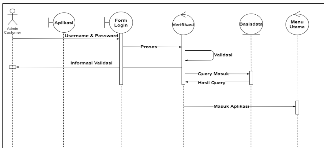
Gambar 5 Sequence Diagram Login
