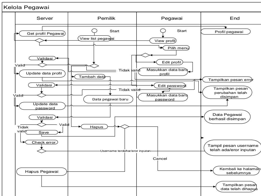
Gambar 1. 2 Activity Diagram Kelola Pegawai
