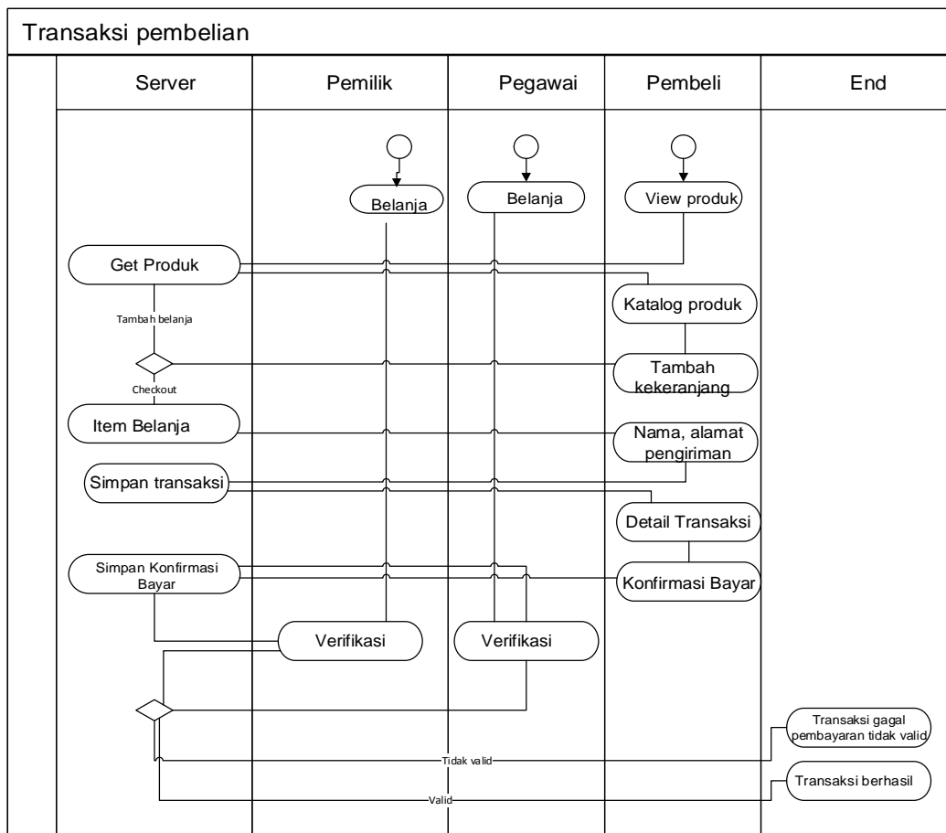
Gambar 1. 4 Activity Diagram Transaksi Pembelian
