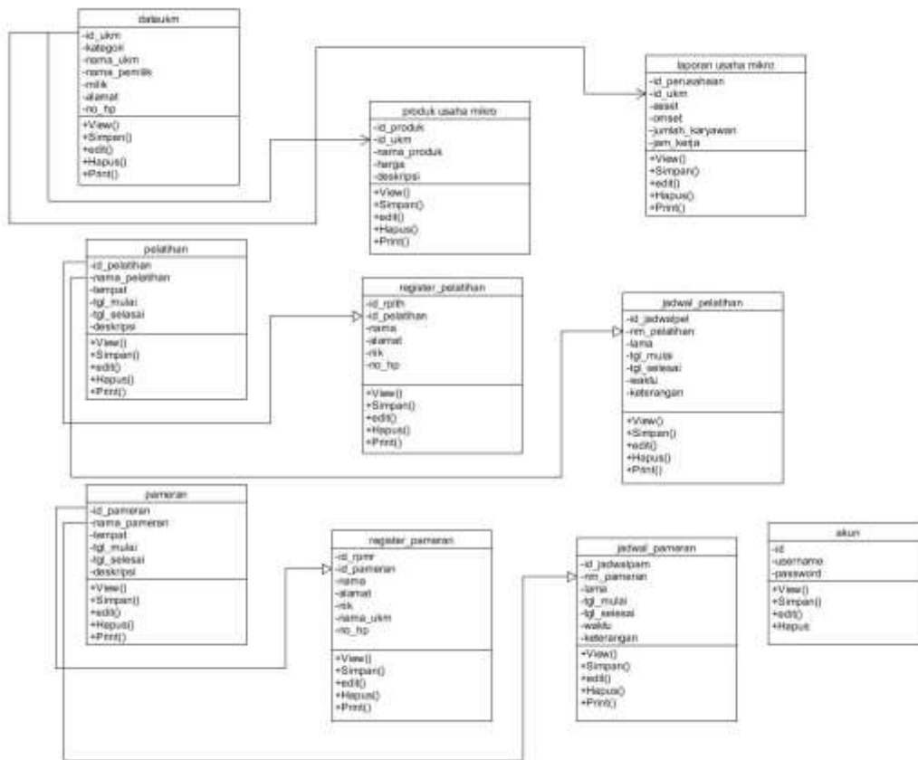
Gambar 1. 3 Class Diagram
