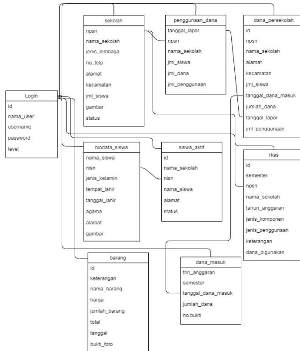
Gambar Class Diagram
