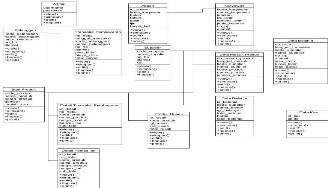
Gambar 1. 4 Class Diagram
