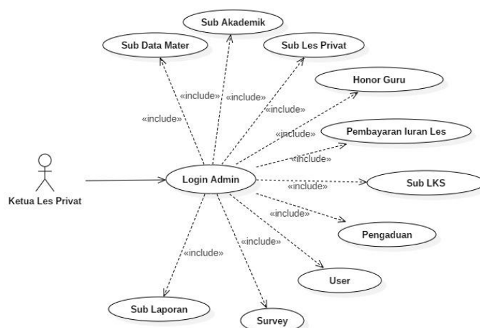
Gambar 1. 3 Use Case Diagram (Admin)
