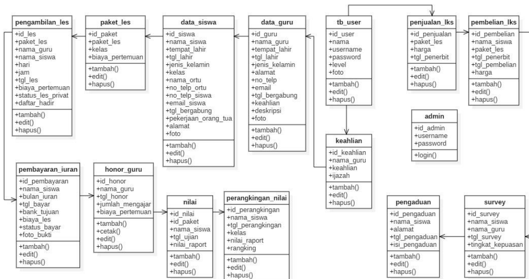
Gambar 1. 6 Class Diagram
