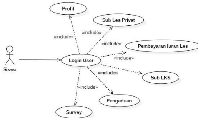
Gambar 1. 5 Use Case Diagram (Siswa)
