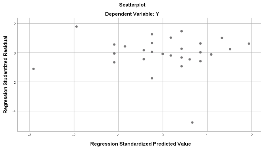
Figure 1. Scatterplot Diagram
