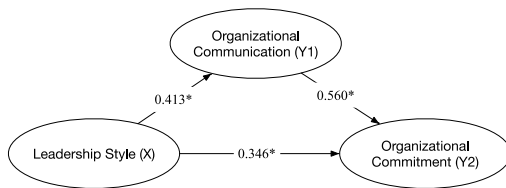
Figure 2. Path diagram of direct analysis
