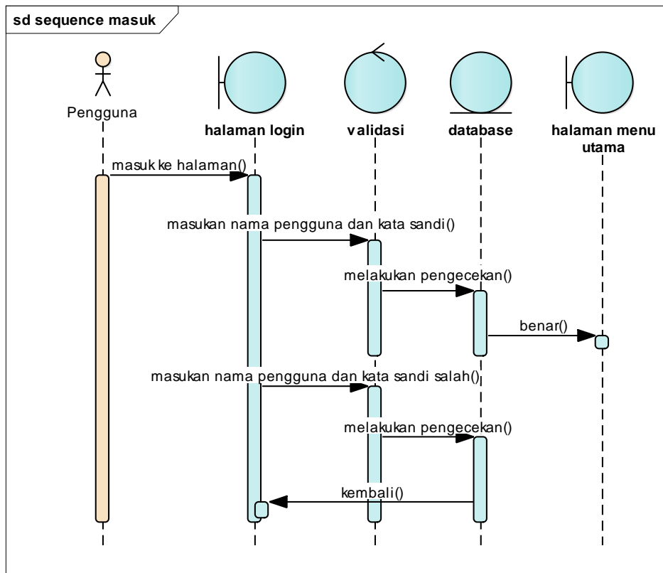
Gambar 4. Sequence Diagram
