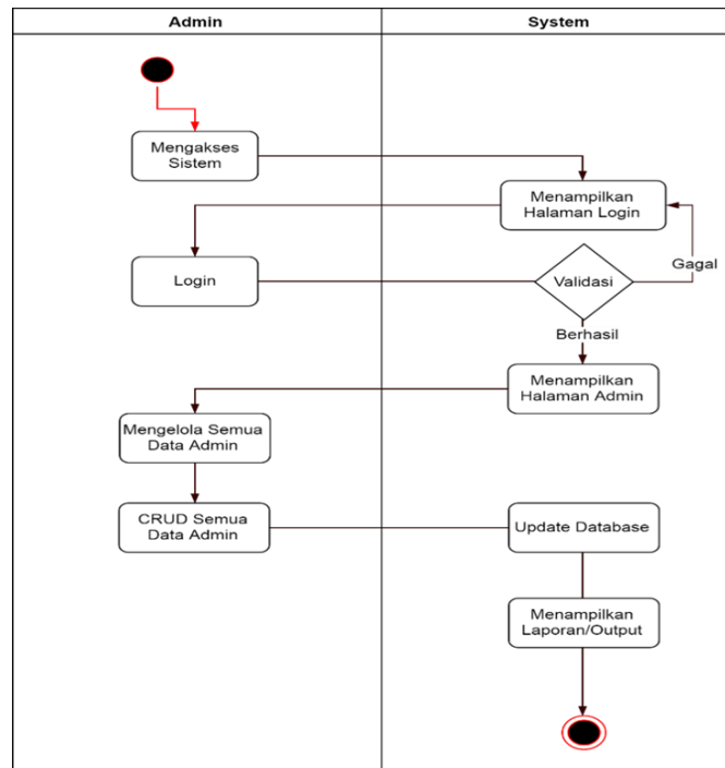
Gambar 3. Activity Diagram
