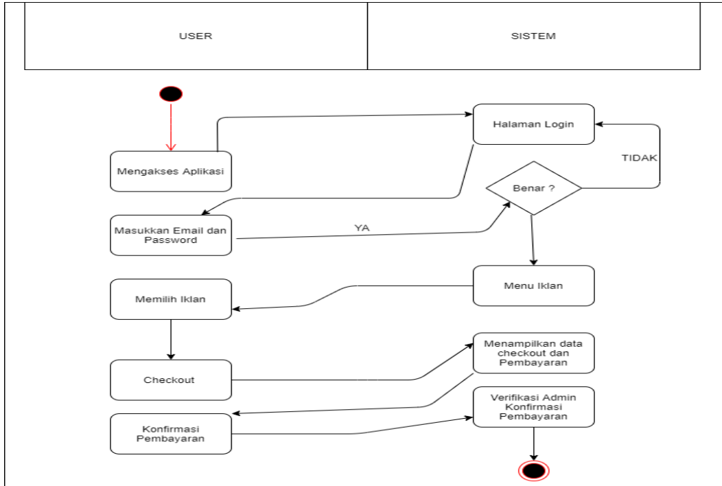
Gambar 3. Activity Diagram User
