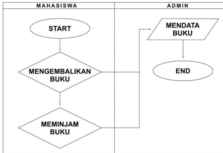
Gambar 1 Flowchart Penelitian
