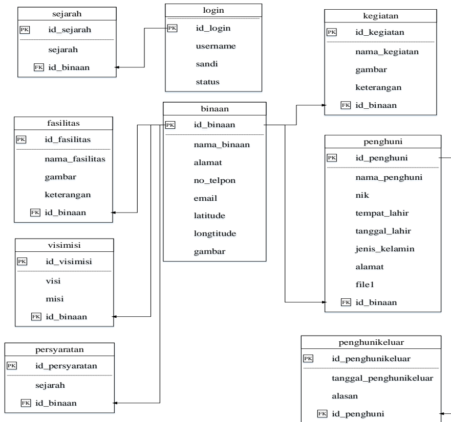
Gambar 15 Class diagram
