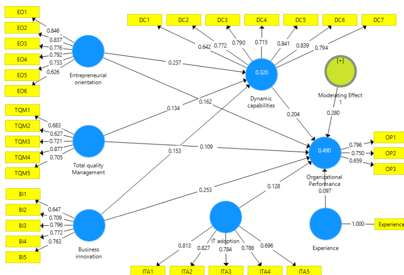
Figure 2. Full Measurement Model
