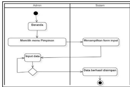
Gambar 4 Activity Diagram Pimpinan
