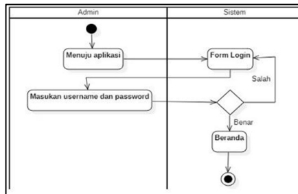
Gambar 5 Activity Diagram Login
