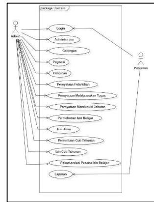
Gambar 1 Usecase Diagram
