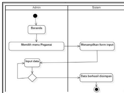
Gambar 6 Activity Diagram Pegawai
