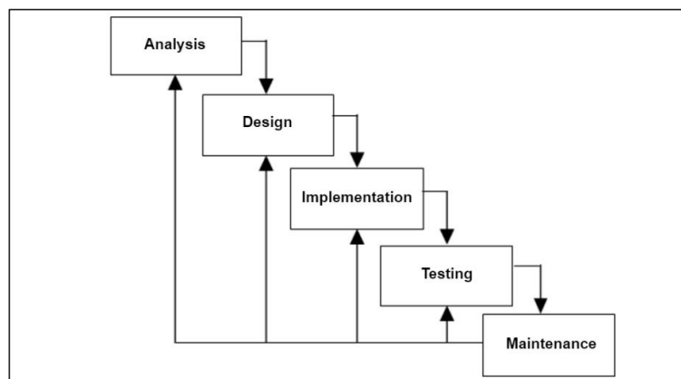
Gambar 1. 1 Metode Waterfall
