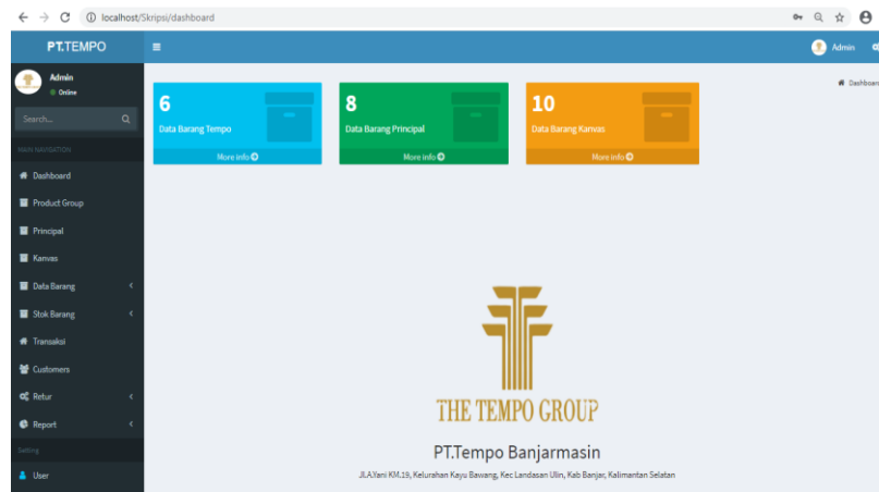
Gambar 4. 2 Form Dashboard
