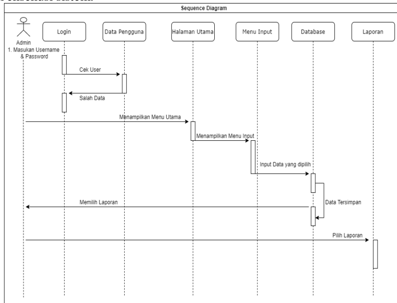
Gambar 3. 8 Sequence Diagram
