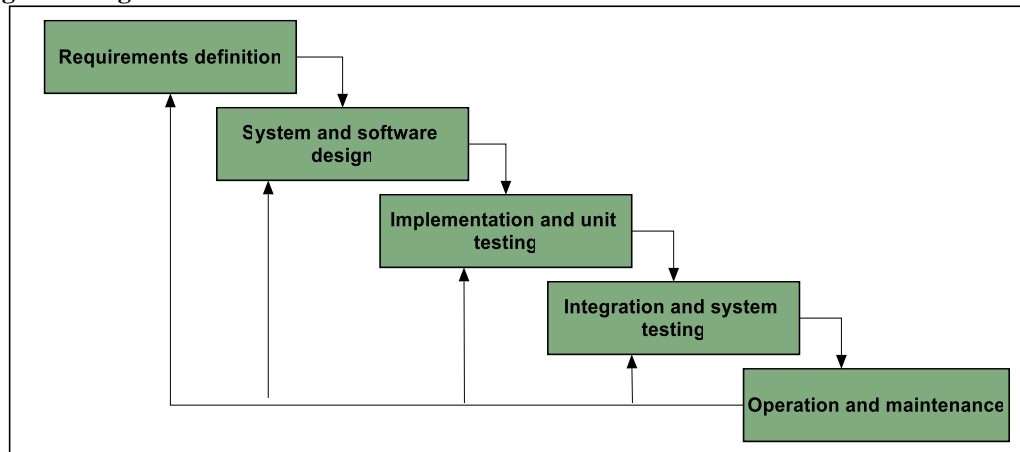
Gambar 1. 1 Model Waterfall
