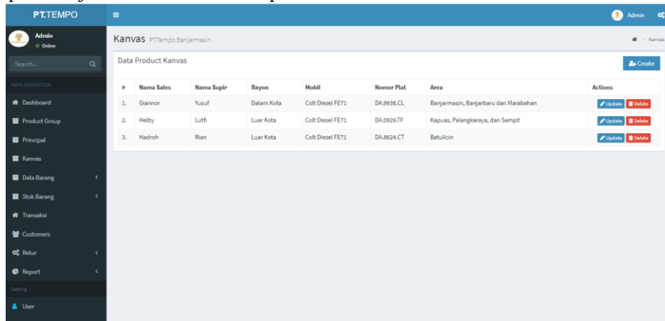
Gambar 4. 7 Form Kanvas
