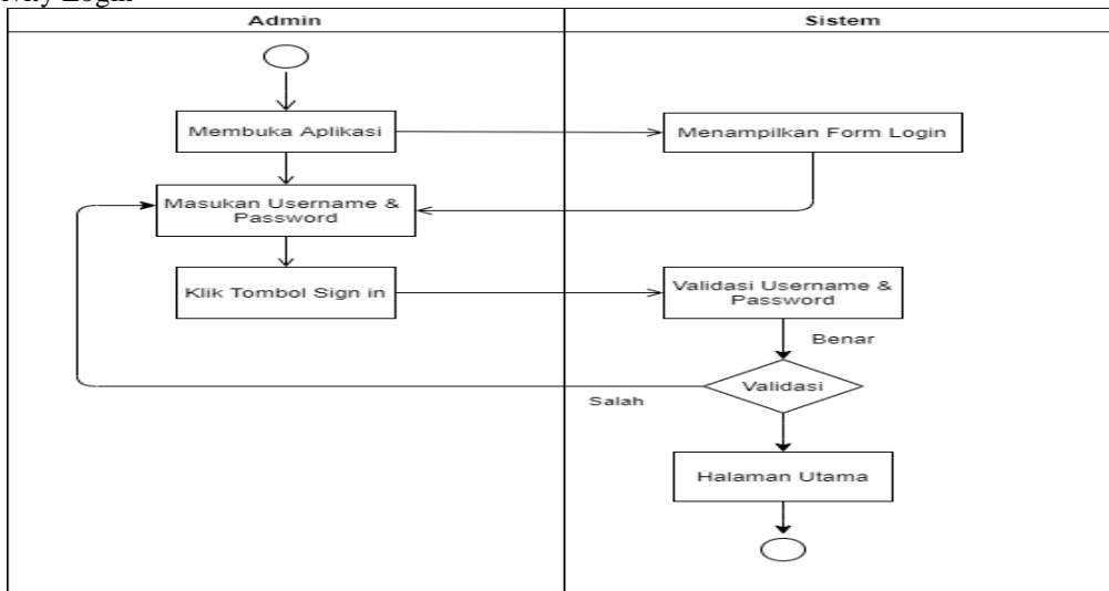
Gambar 3. 4 Activity Login
