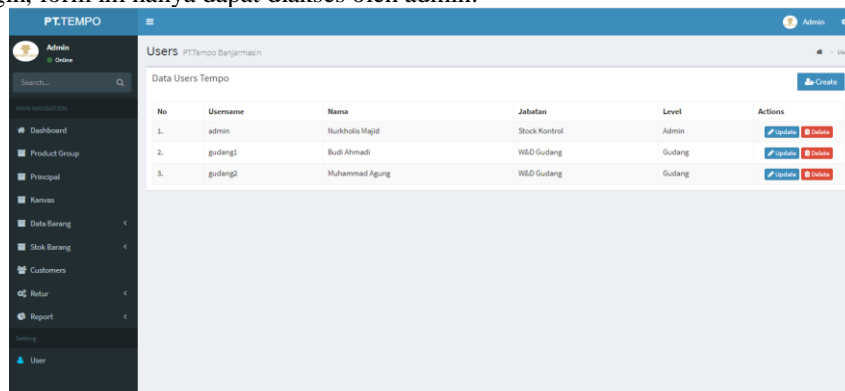
Gambar 4. 3 Form User
