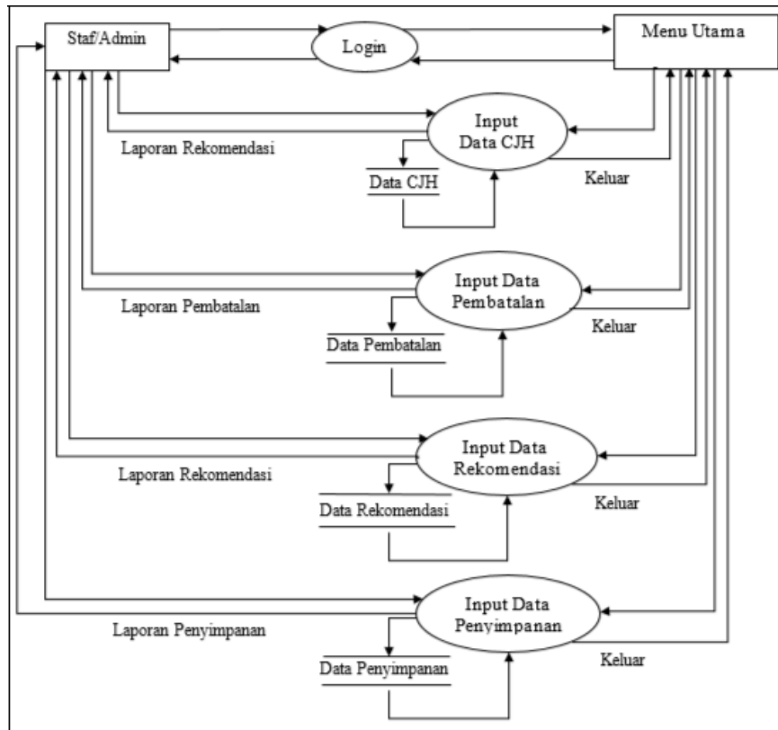
Gambar 3. DFD Level 1
