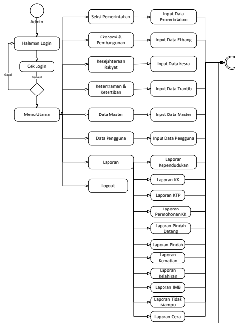
Gambar 3. 3 Diagram Activity
