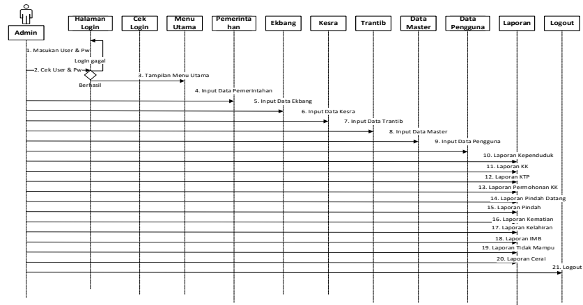
Gambar 3. 5 Sequence Diagram Admin
